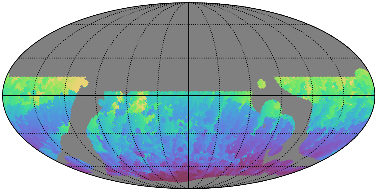
telescope_jerk_v3.5_10yrs WFD i band: Min HA
