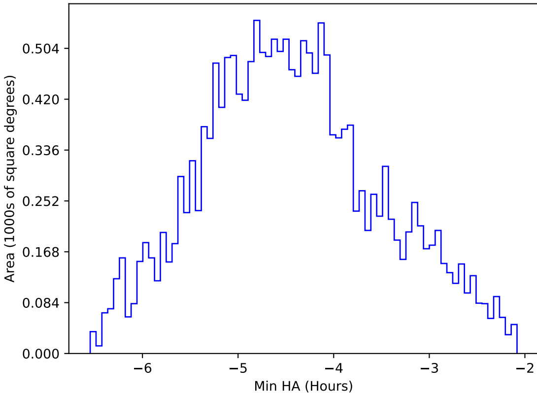
telescope_jerk_v3.5_10yrs WFD i band: Min HA
