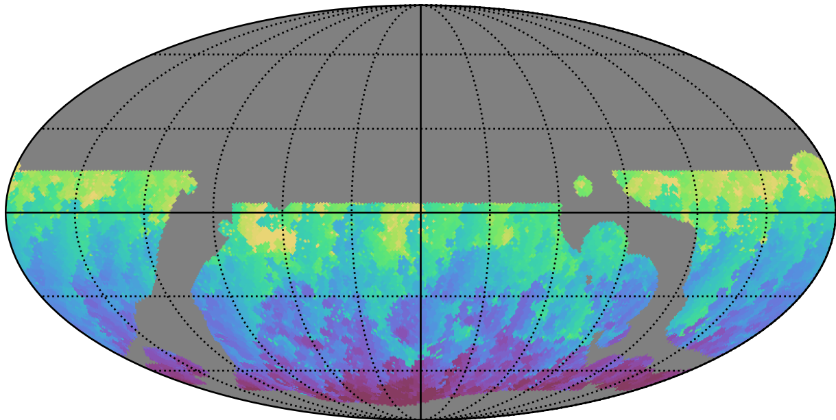
telescope_jerk_v3.5_10yrs WFD g band: Min HA
