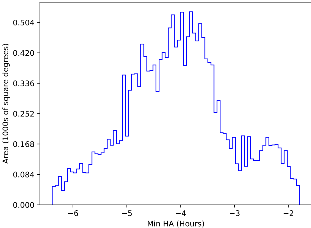
telescope_jerk_v3.5_10yrs WFD g band: Min HA
