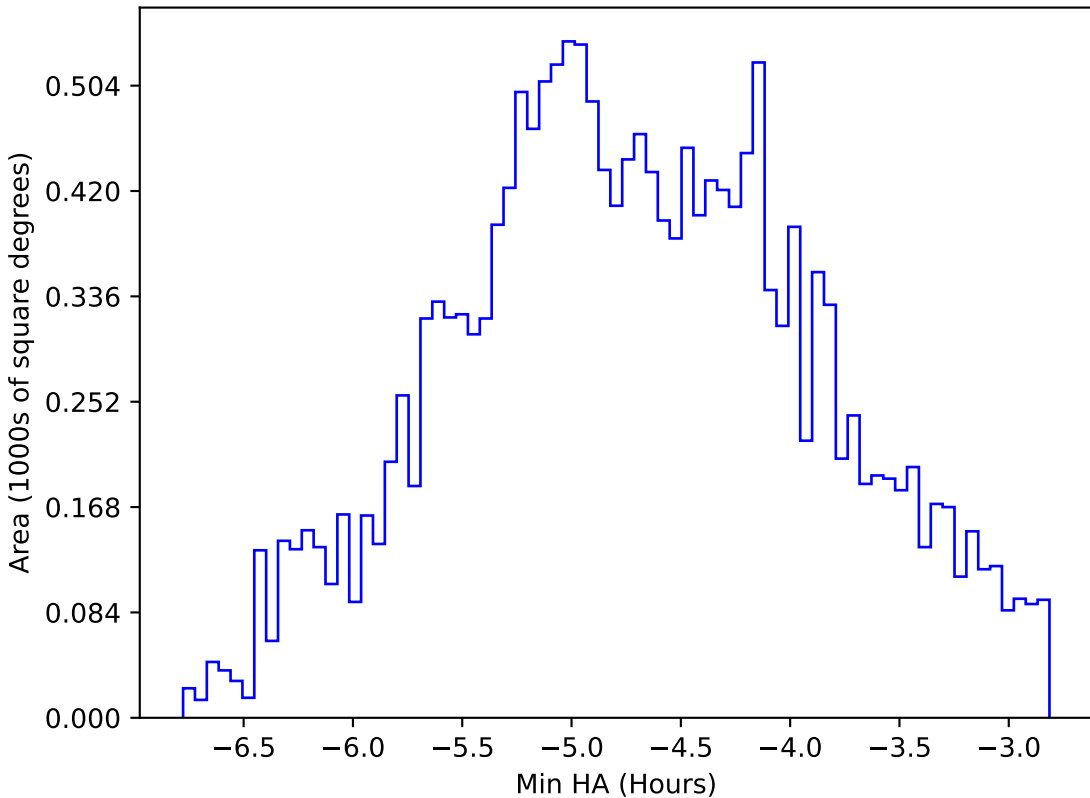
telescope_jerk_v3.5_10yrs WFD all bands: Min HA
