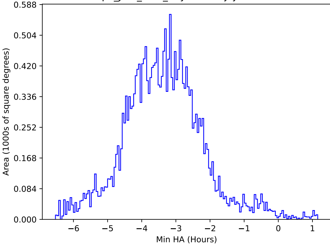
telescope_jerk_v3.5_10yrs All sky y band: Min HA
