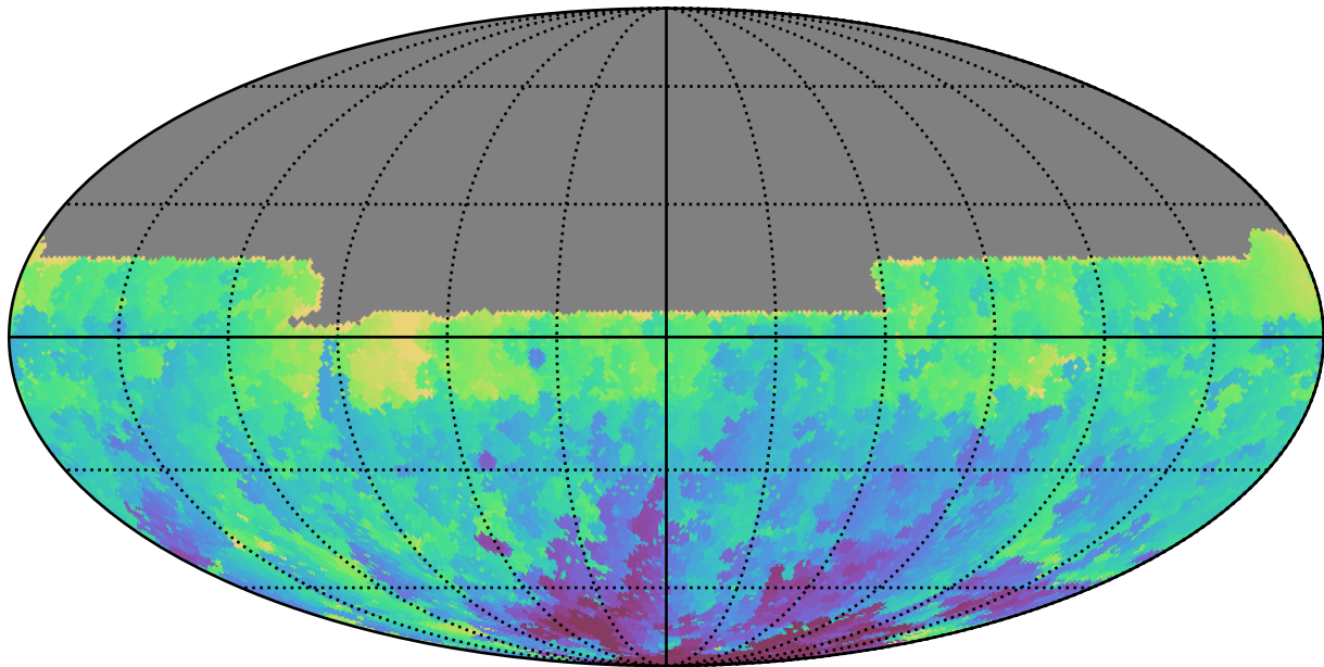
telescope_jerk_v3.5_10yrs All sky u band: Min HA
