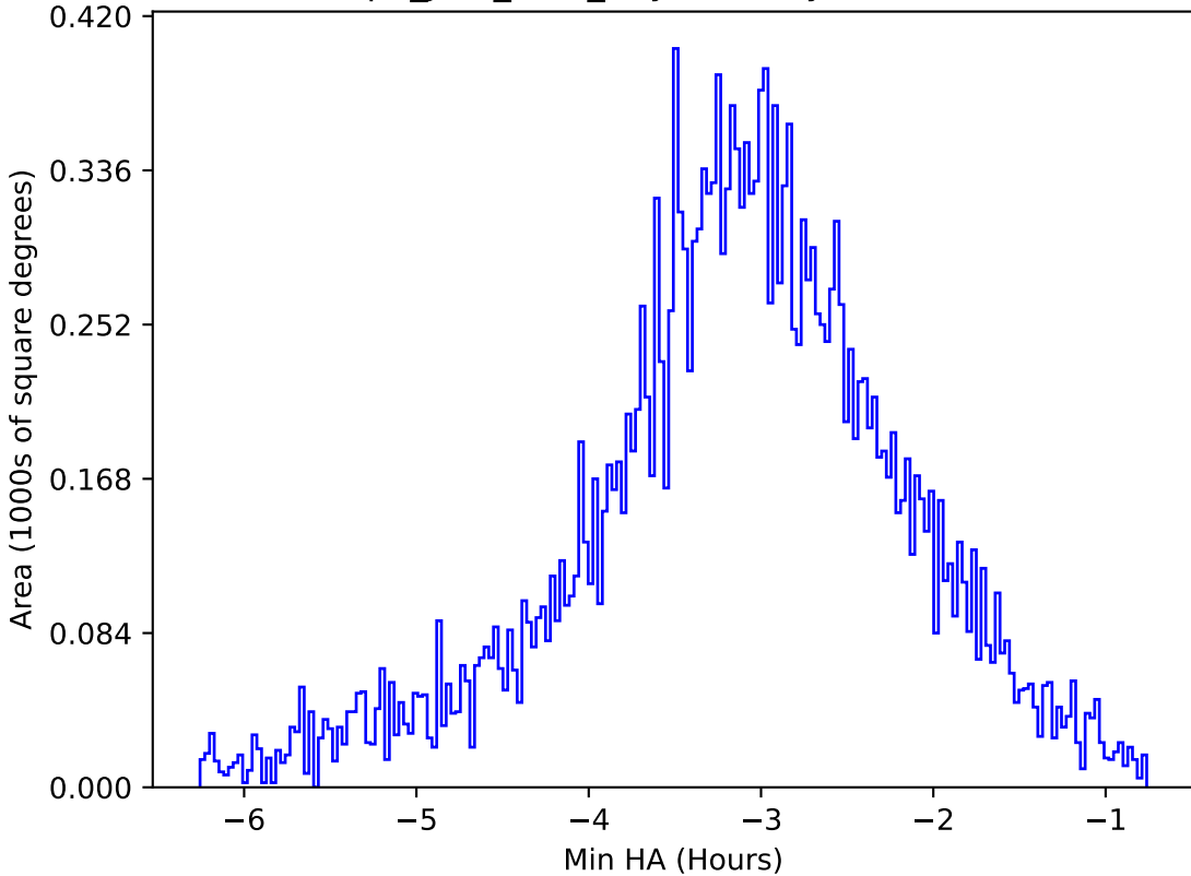
telescope_jerk_v3.5_10yrs All sky u band: Min HA
