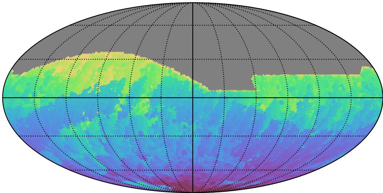
telescope_jerk_v3.5_10yrs All sky i band: Min HA
