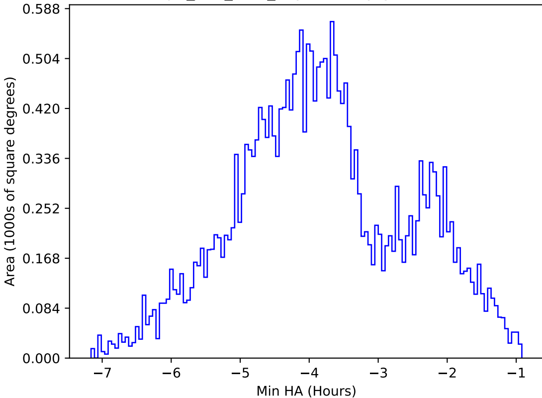
telescope_jerk_v3.5_10yrs All sky g band: Min HA
