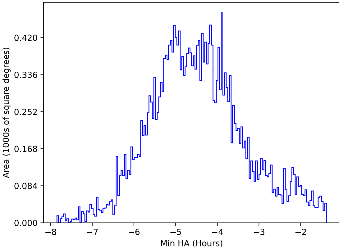
telescope_jerk_v3.5_10yrs All sky all bands: Min HA
