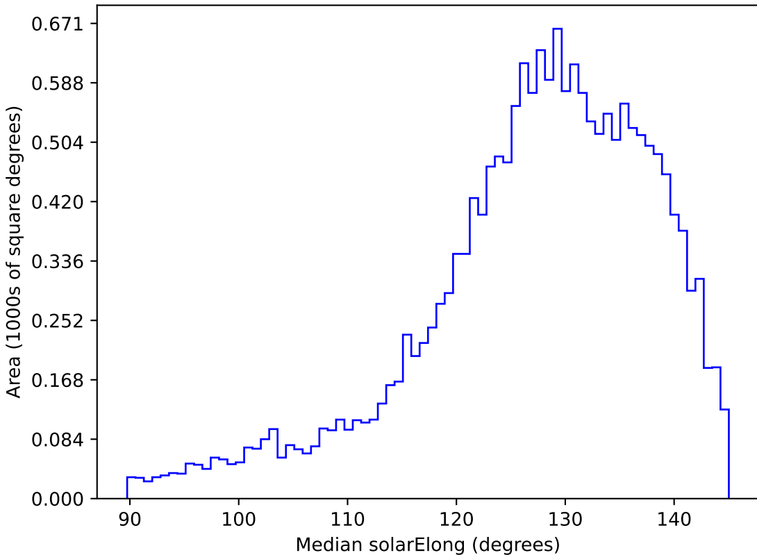
telescope_jerk_v3.5_10yrs WFD z band: Median solarElong
