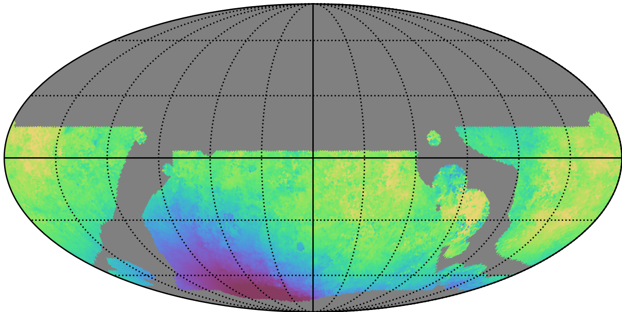
telescope_jerk_v3.5_10yrs WFD y band: Median solarElong
