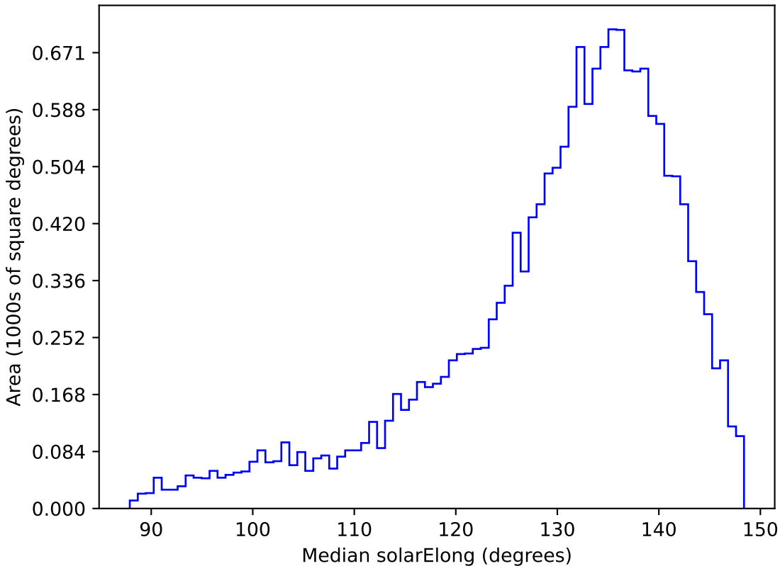
telescope_jerk_v3.5_10yrs WFD y band: Median solarElong
