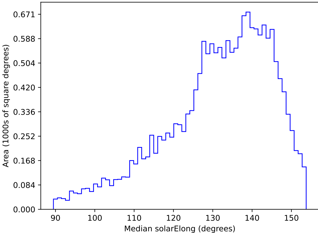
telescope_jerk_v3.5_10yrs WFD u band: Median solarElong
