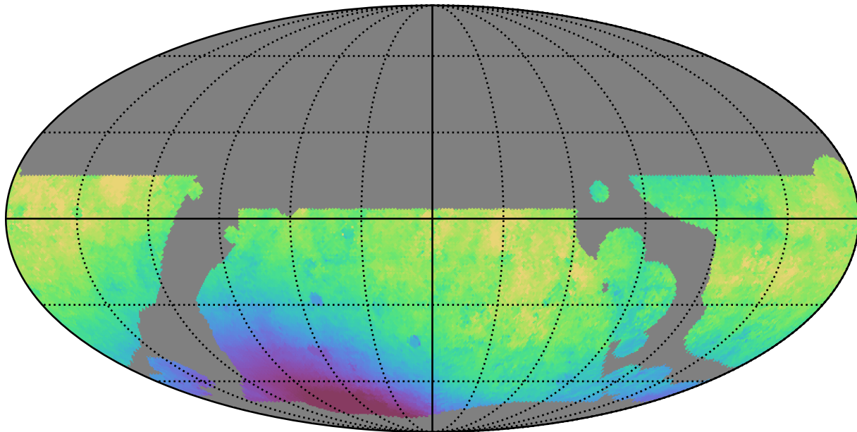
telescope_jerk_v3.5_10yrs WFD r band: Median solarElong
