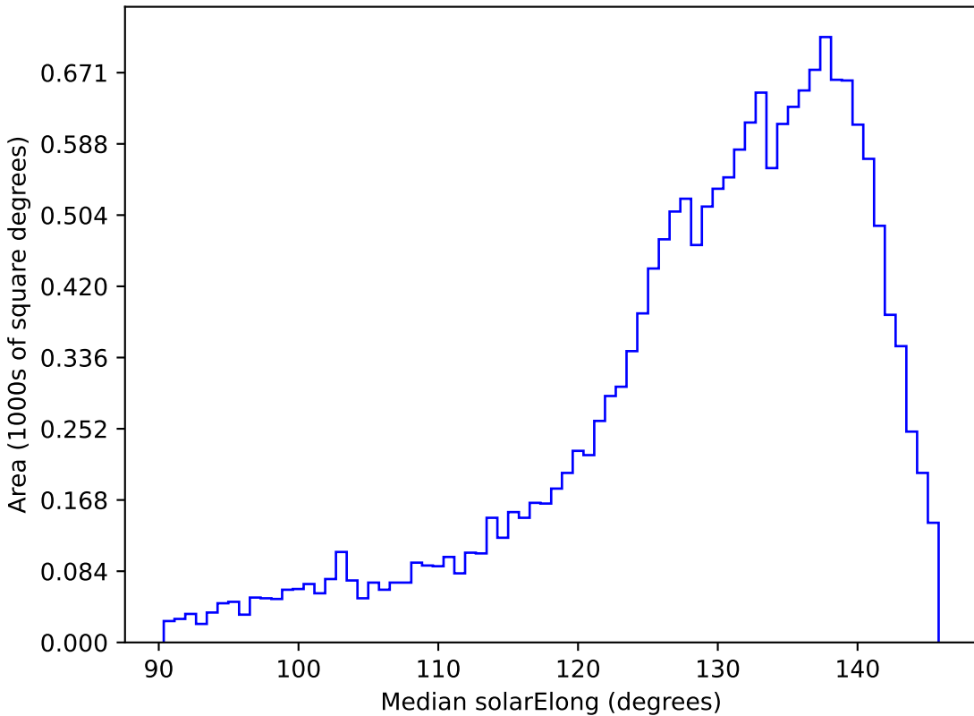
telescope_jerk_v3.5_10yrs WFD r band: Median solarElong
