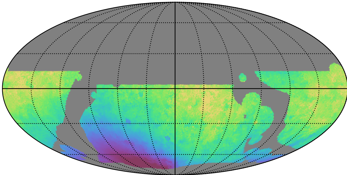
telescope_jerk_v3.5_10yrs WFD i band: Median solarElong
