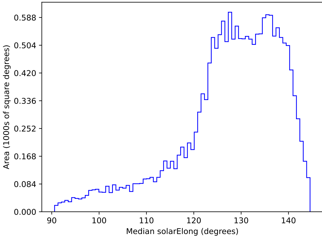
telescope_jerk_v3.5_10yrs WFD i band: Median solarElong
