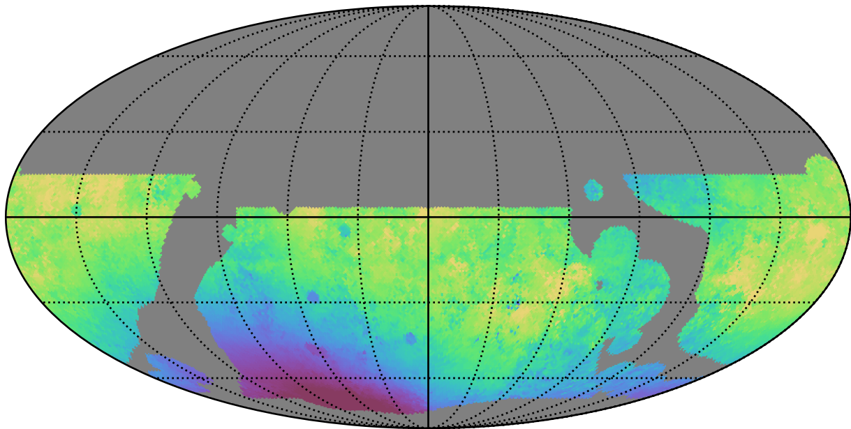
telescope_jerk_v3.5_10yrs WFD g band: Median solarElong
