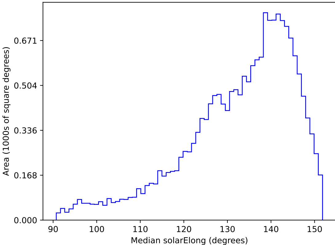
telescope_jerk_v3.5_10yrs WFD g band: Median solarElong
