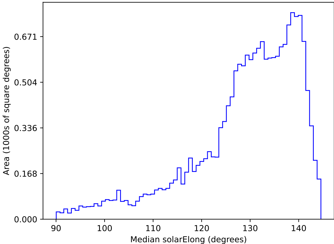
telescope_jerk_v3.5_10yrs WFD all bands: Median solarElong
