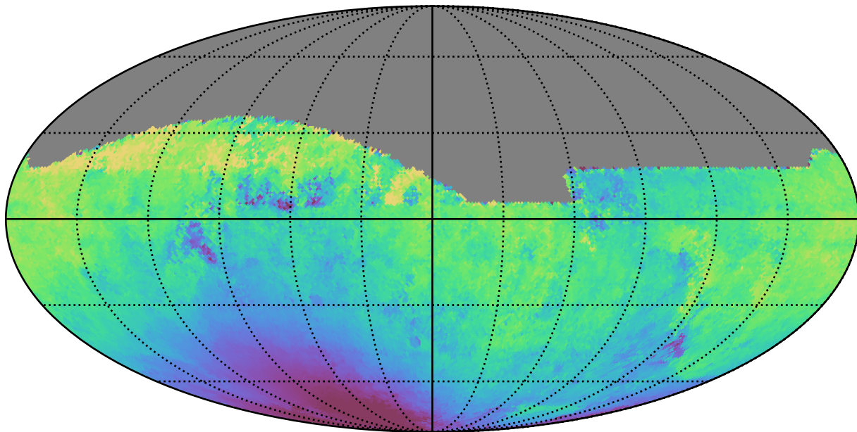
telescope_jerk_v3.5_10yrs All sky z band: Median solarElong
