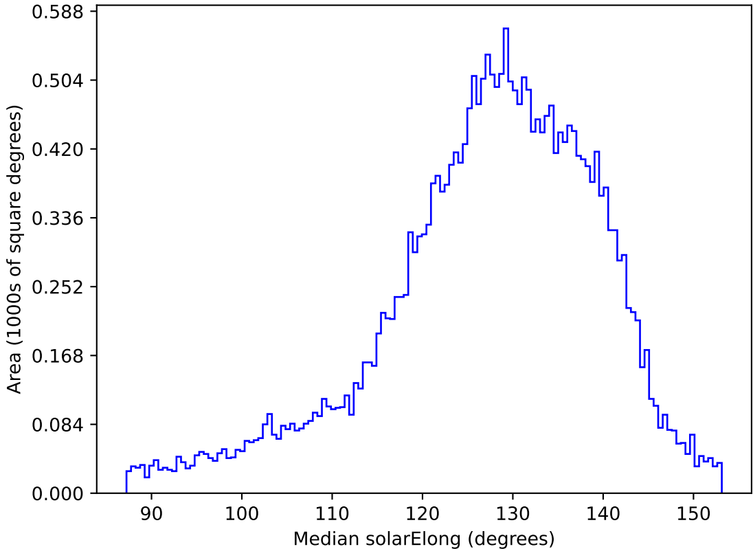
telescope_jerk_v3.5_10yrs All sky z band: Median solarElong
