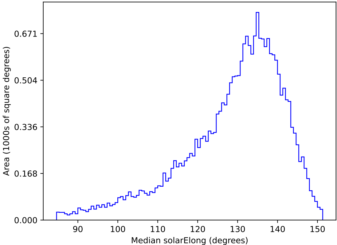
telescope_jerk_v3.5_10yrs All sky y band: Median solarElong
