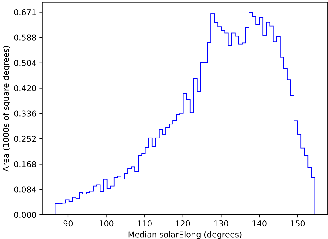
telescope_jerk_v3.5_10yrs All sky u band: Median solarElong
