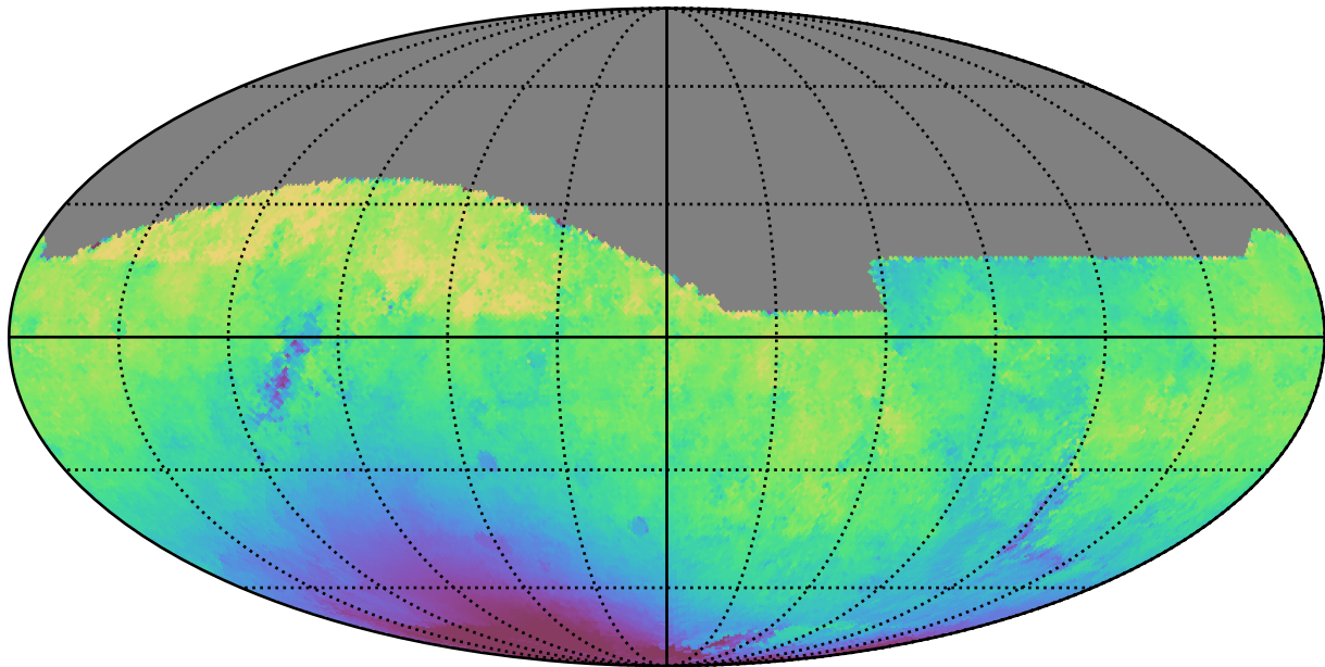
telescope_jerk_v3.5_10yrs All sky r band: Median solarElong
