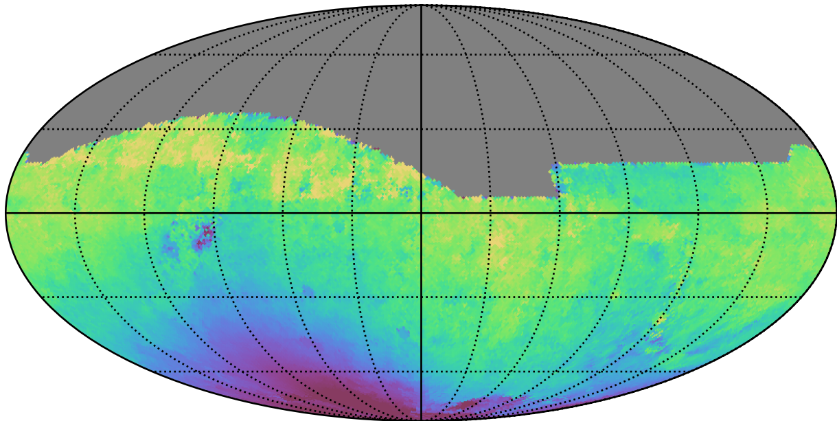
telescope_jerk_v3.5_10yrs All sky i band: Median solarElong
