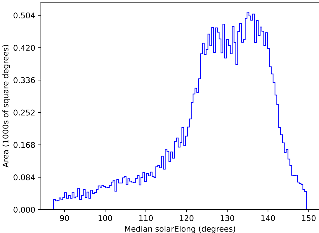
telescope_jerk_v3.5_10yrs All sky i band: Median solarElong
