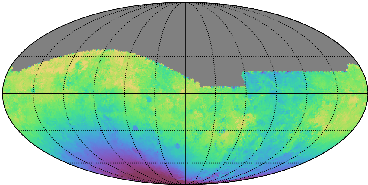
telescope_jerk_v3.5_10yrs All sky g band: Median solarElong
