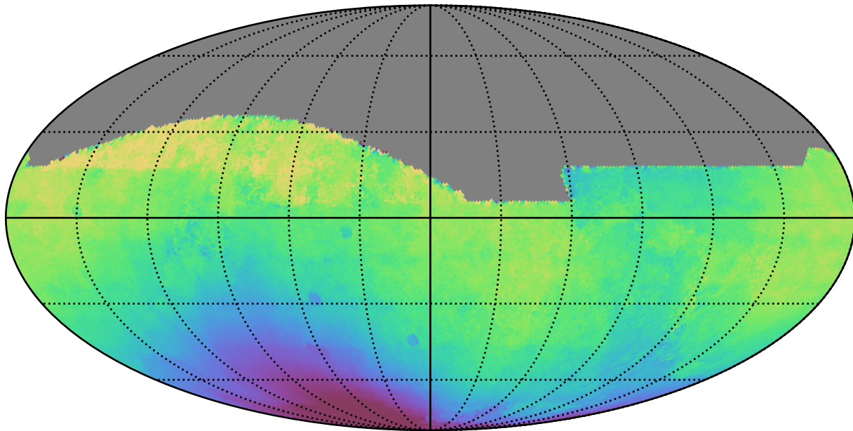
telescope_jerk_v3.5_10yrs All sky all bands: Median solarElong
