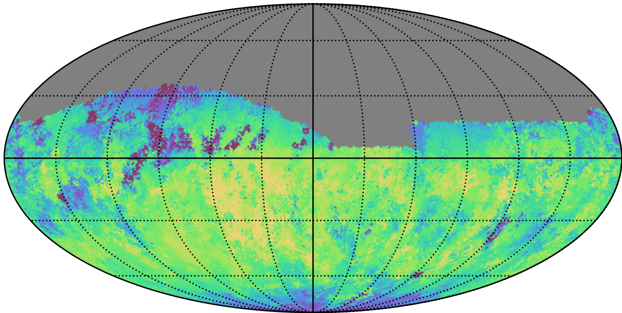
telescope_jerk_v3.5_10yrs Yr 1 z band: Median skyBrightness
