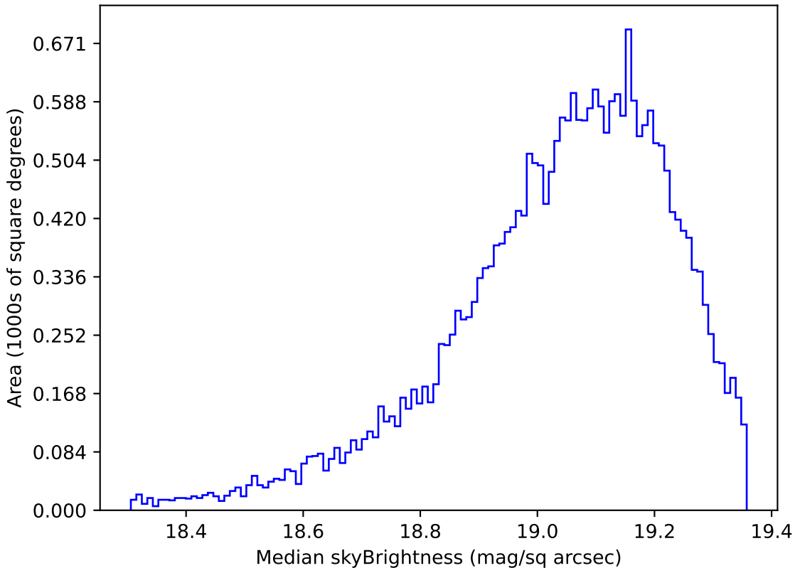
telescope_jerk_v3.5_10yrs Yr 1 z band: Median skyBrightness
