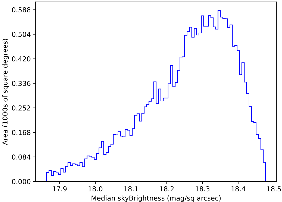
telescope_jerk_v3.5_10yrs Yr 1 y band: Median skyBrightness
