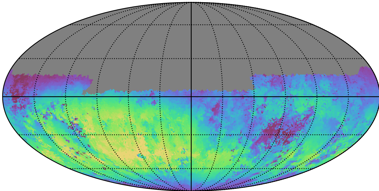
telescope_jerk_v3.5_10yrs Yr 1 u band: Median skyBrightness
