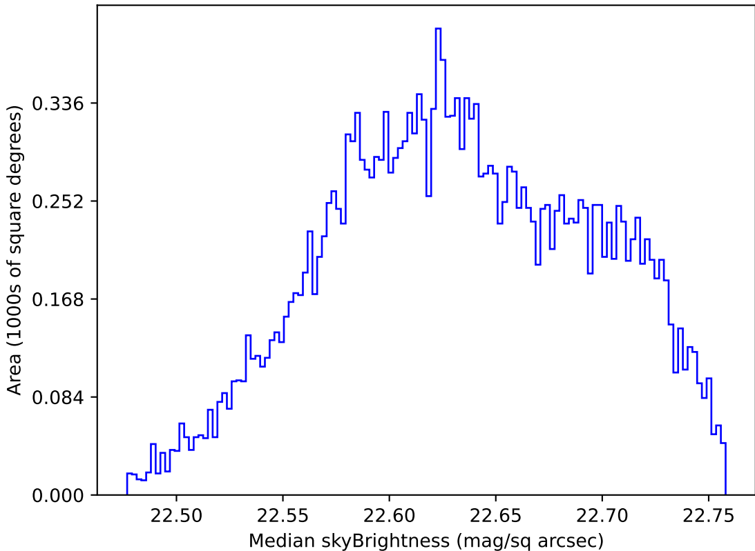
telescope_jerk_v3.5_10yrs Yr 1 u band: Median skyBrightness
