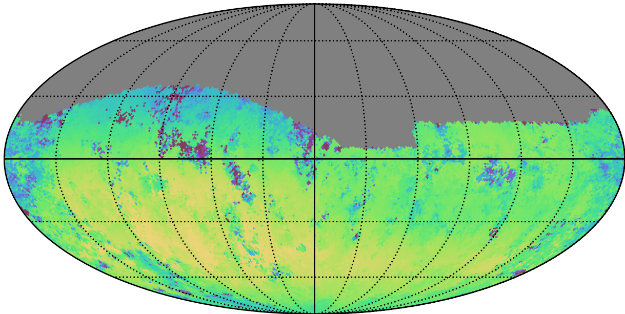
telescope_jerk_v3.5_10yrs Yr 1 r band: Median skyBrightness
