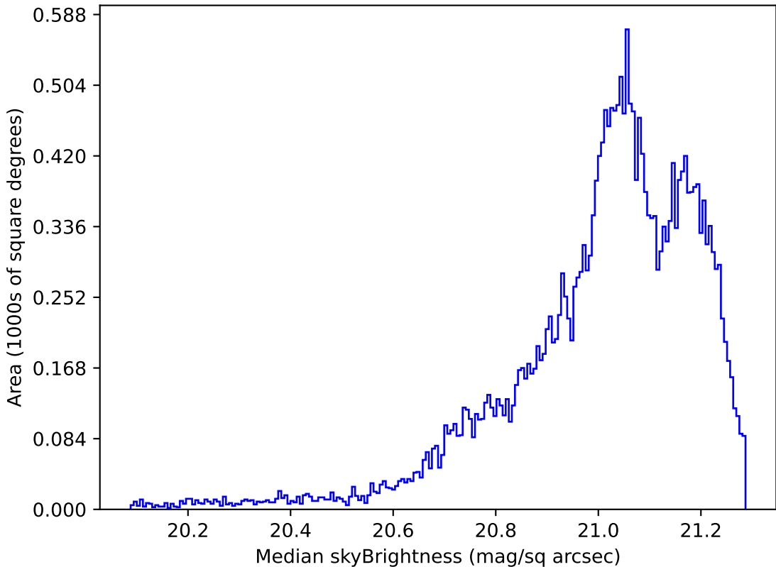
telescope_jerk_v3.5_10yrs Yr 1 r band: Median skyBrightness
