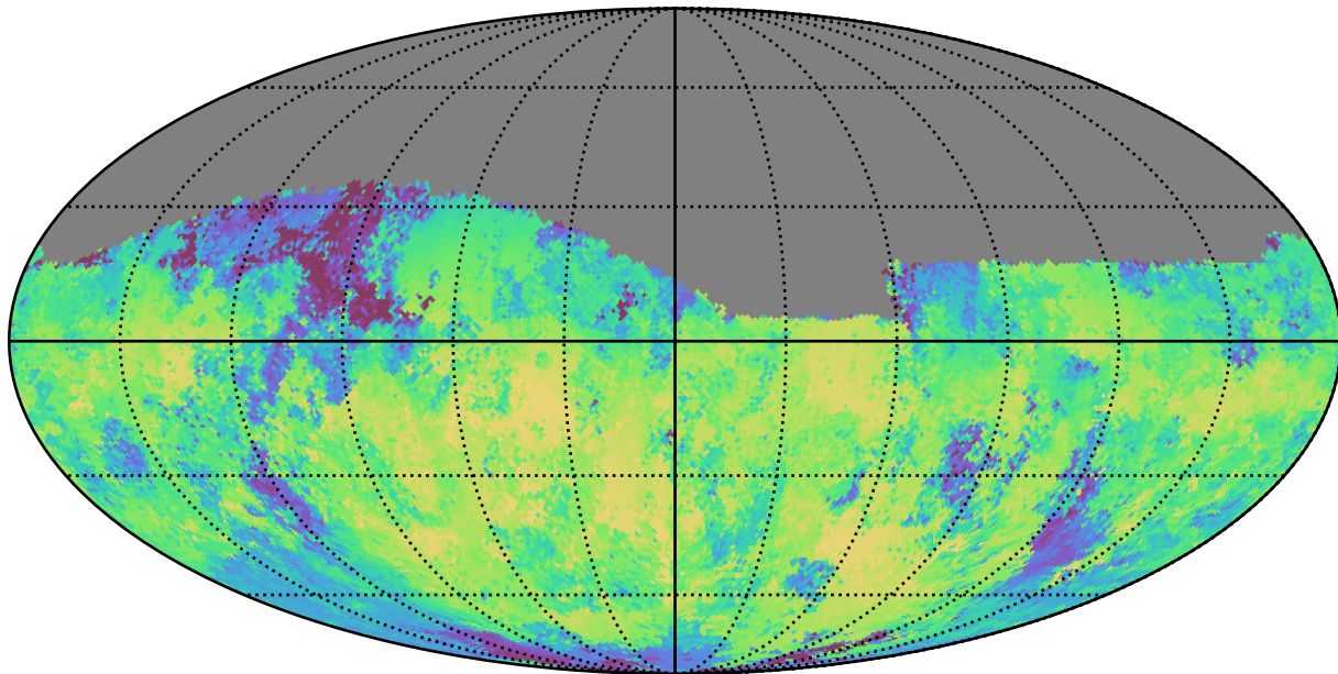
telescope_jerk_v3.5_10yrs Yr 1 i band: Median skyBrightness
