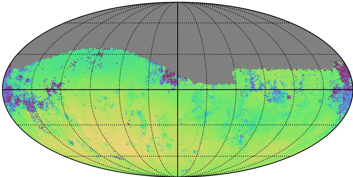
telescope_jerk_v3.5_10yrs Yr 1 g band: Median skyBrightness
