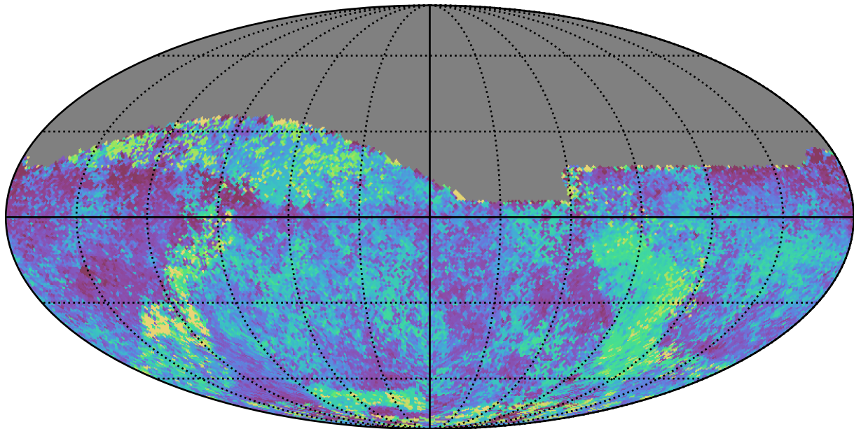
telescope_jerk_v3.5_10yrs Yr 1 all bands: Median skyBrightness
