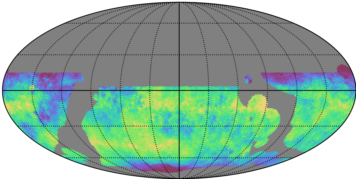
telescope_jerk_v3.5_10yrs WFD z band: Median skyBrightness
