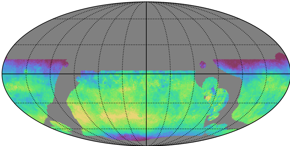
telescope_jerk_v3.5_10yrs WFD y band: Median skyBrightness
