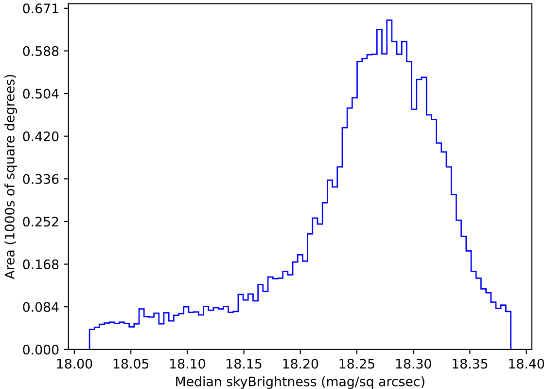
telescope_jerk_v3.5_10yrs WFD y band: Median skyBrightness
