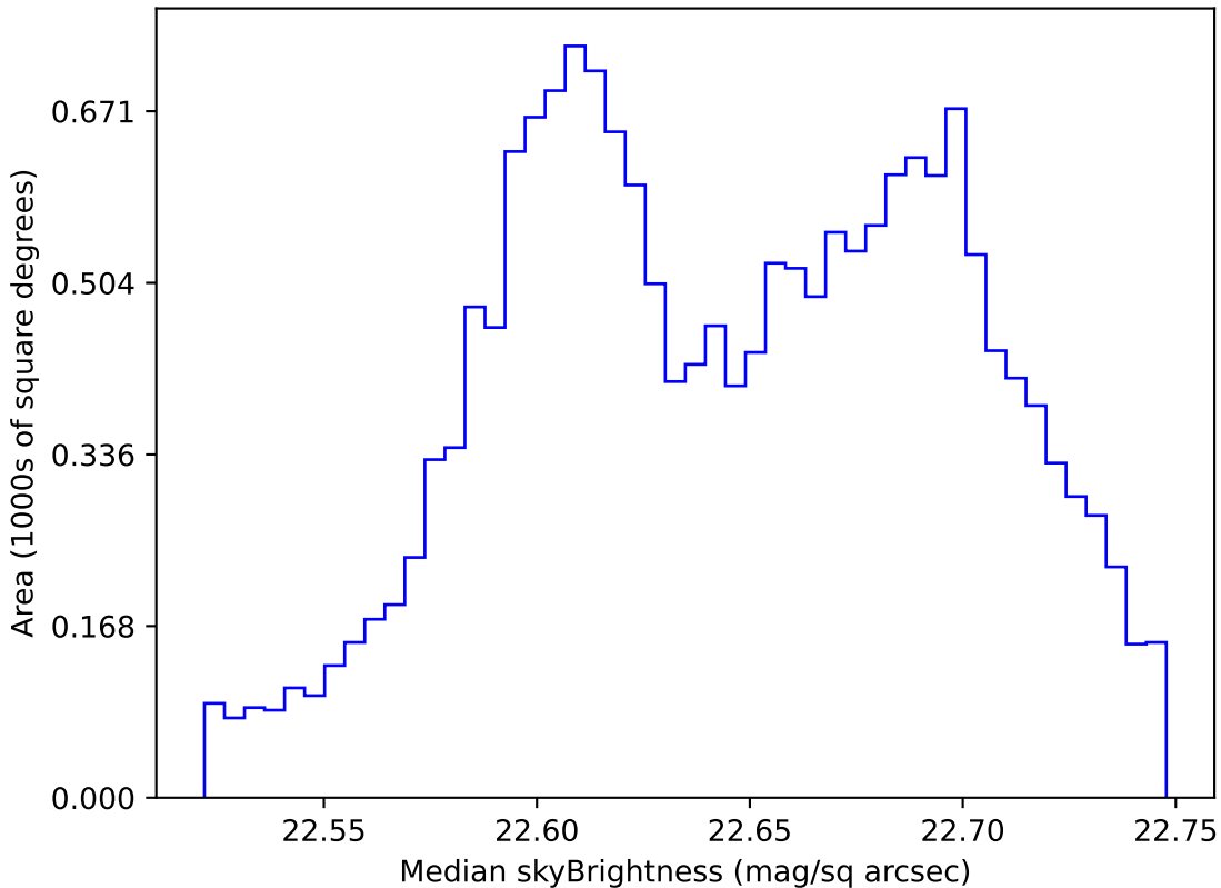
telescope_jerk_v3.5_10yrs WFD u band: Median skyBrightness
