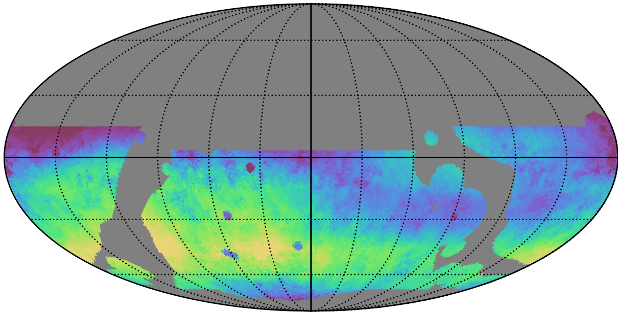
telescope_jerk_v3.5_10yrs WFD r band: Median skyBrightness
