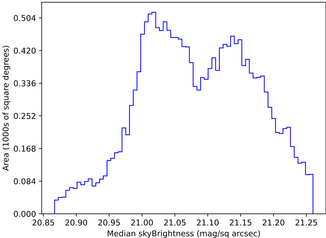
telescope_jerk_v3.5_10yrs WFD r band: Median skyBrightness
