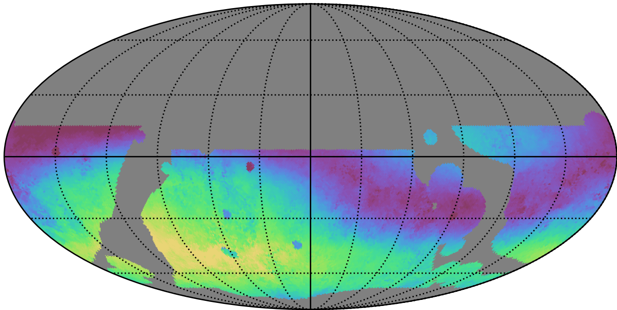
telescope_jerk_v3.5_10yrs WFD g band: Median skyBrightness
