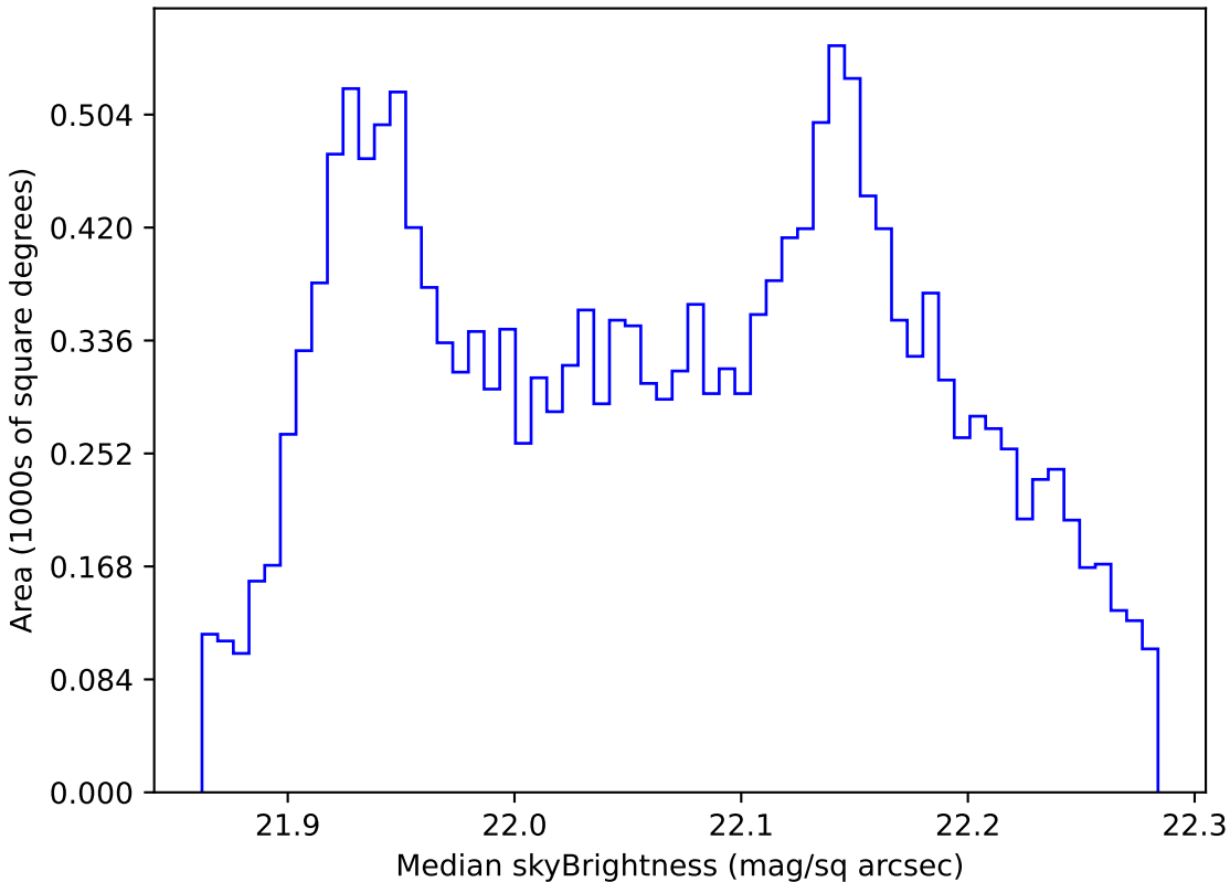
telescope_jerk_v3.5_10yrs WFD g band: Median skyBrightness
