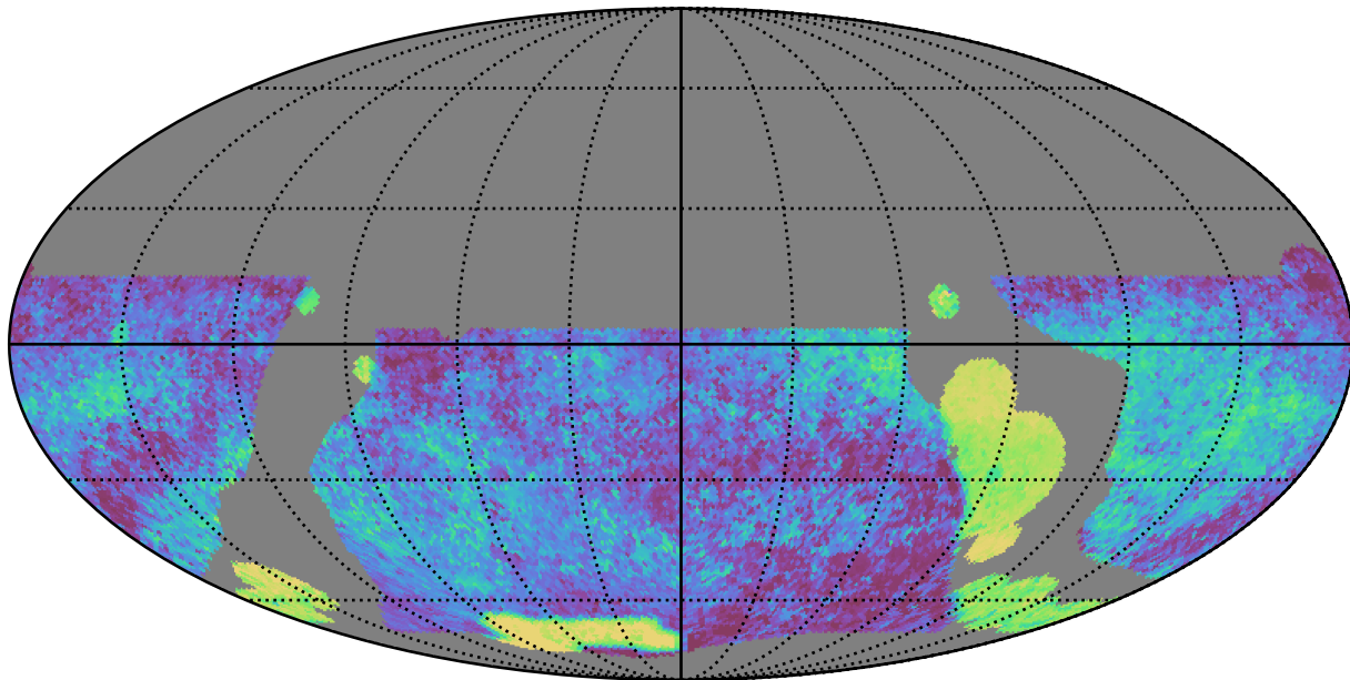
telescope_jerk_v3.5_10yrs WFD all bands: Median skyBrightness
